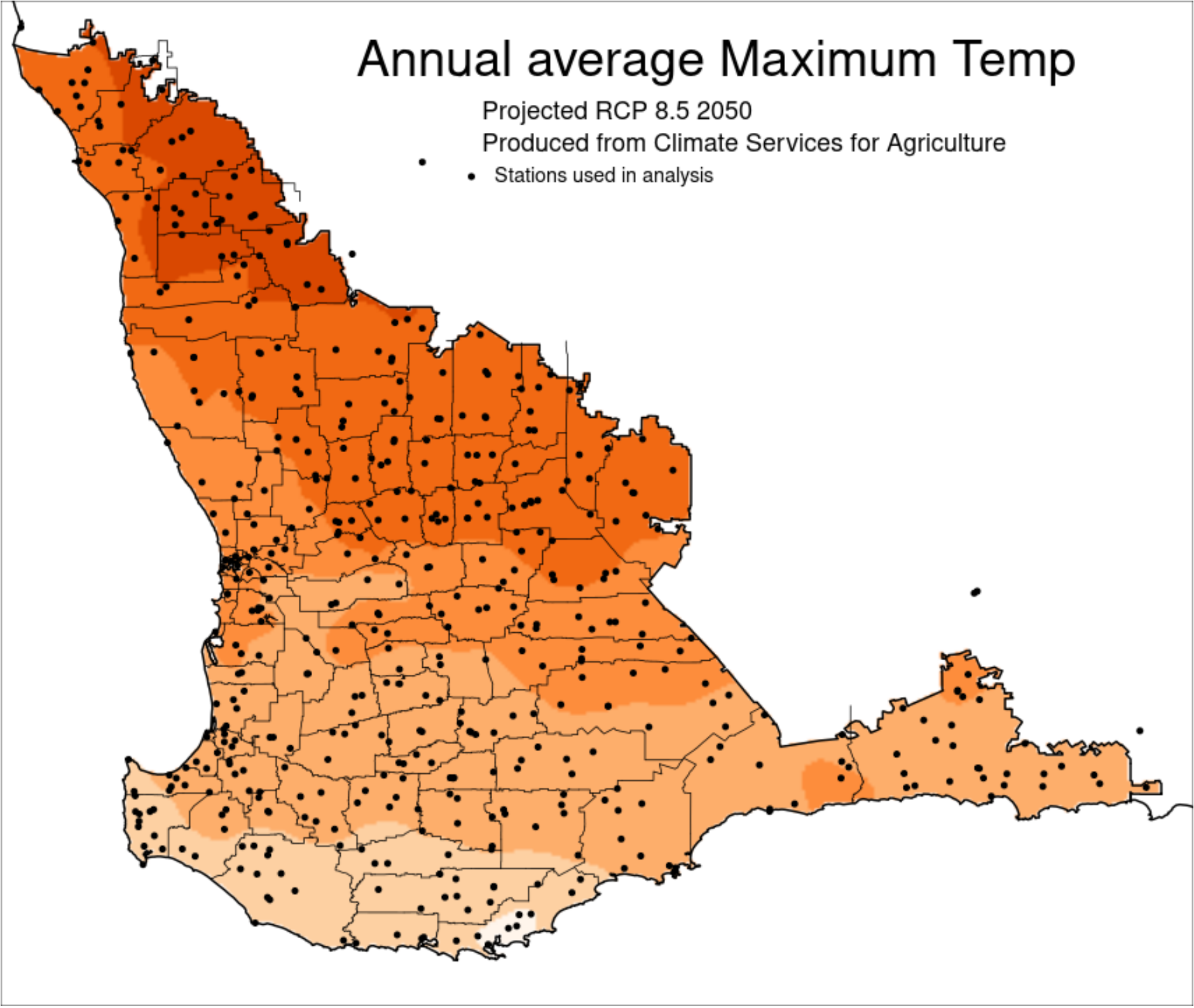
RCP 8.5 2050
