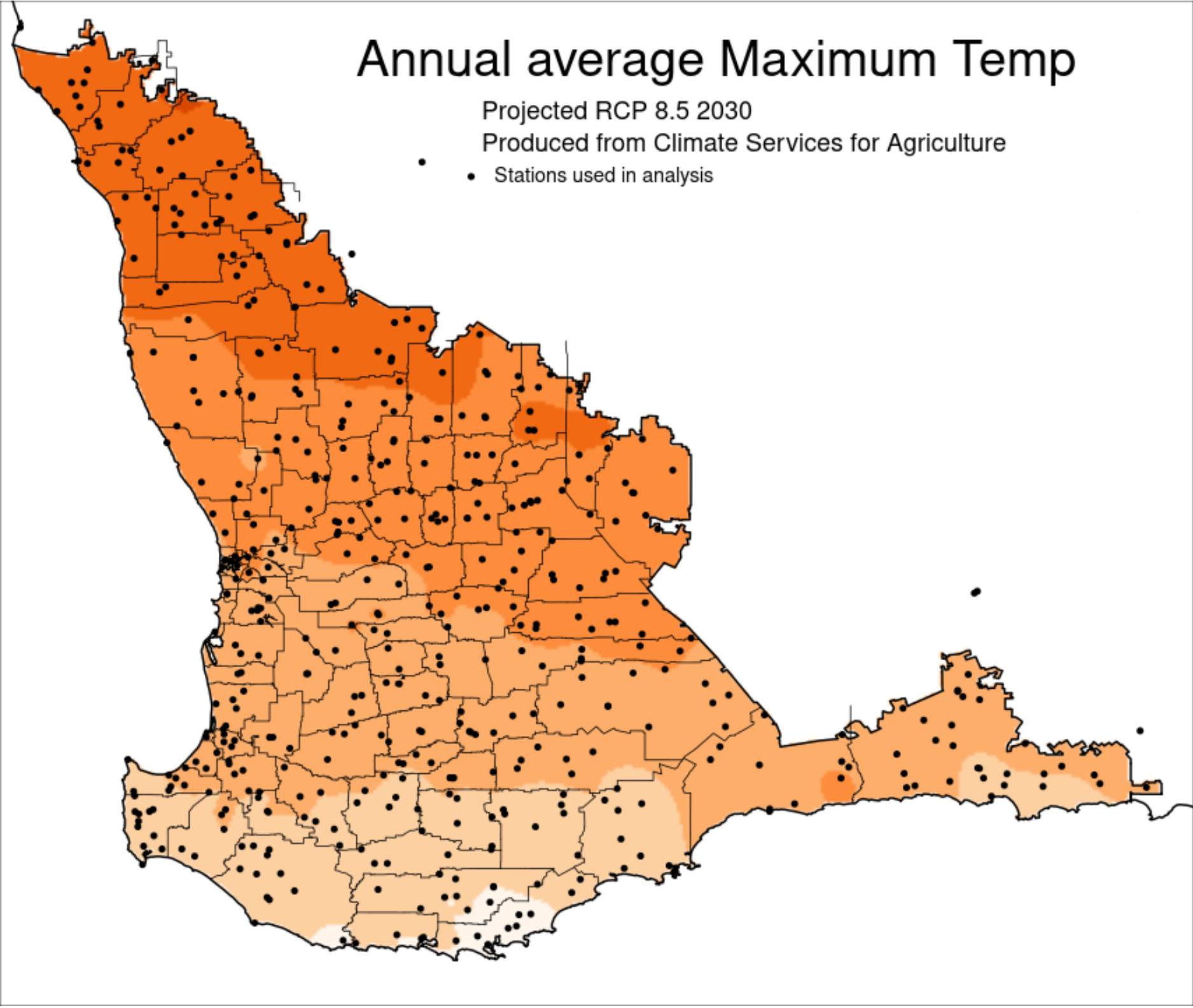
RCP 8.5 2030
