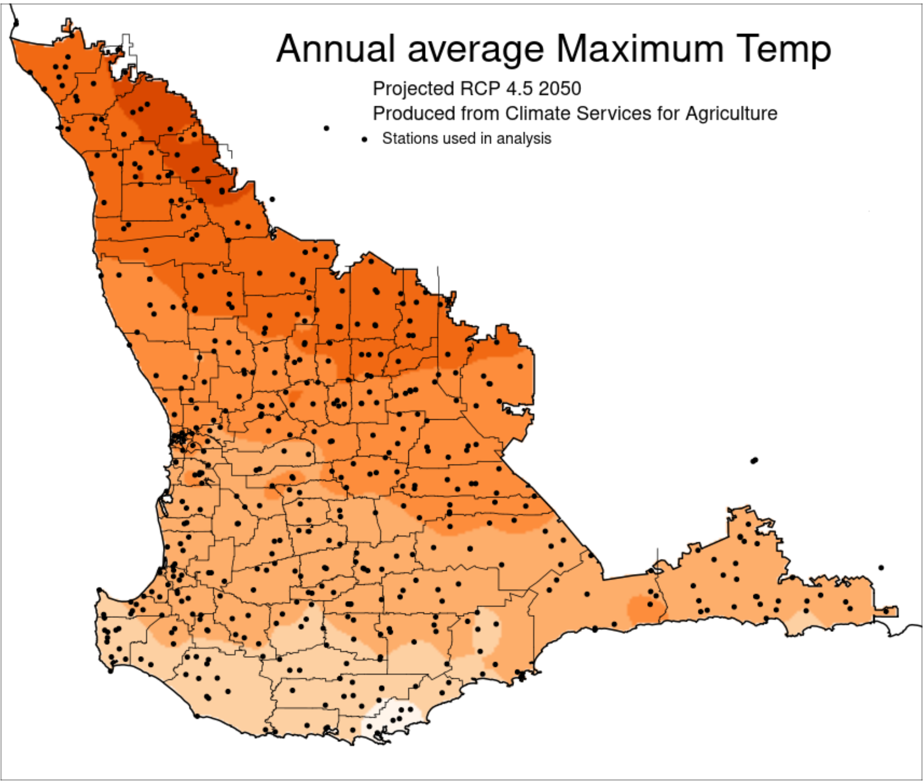
RCP 4.5 2050
