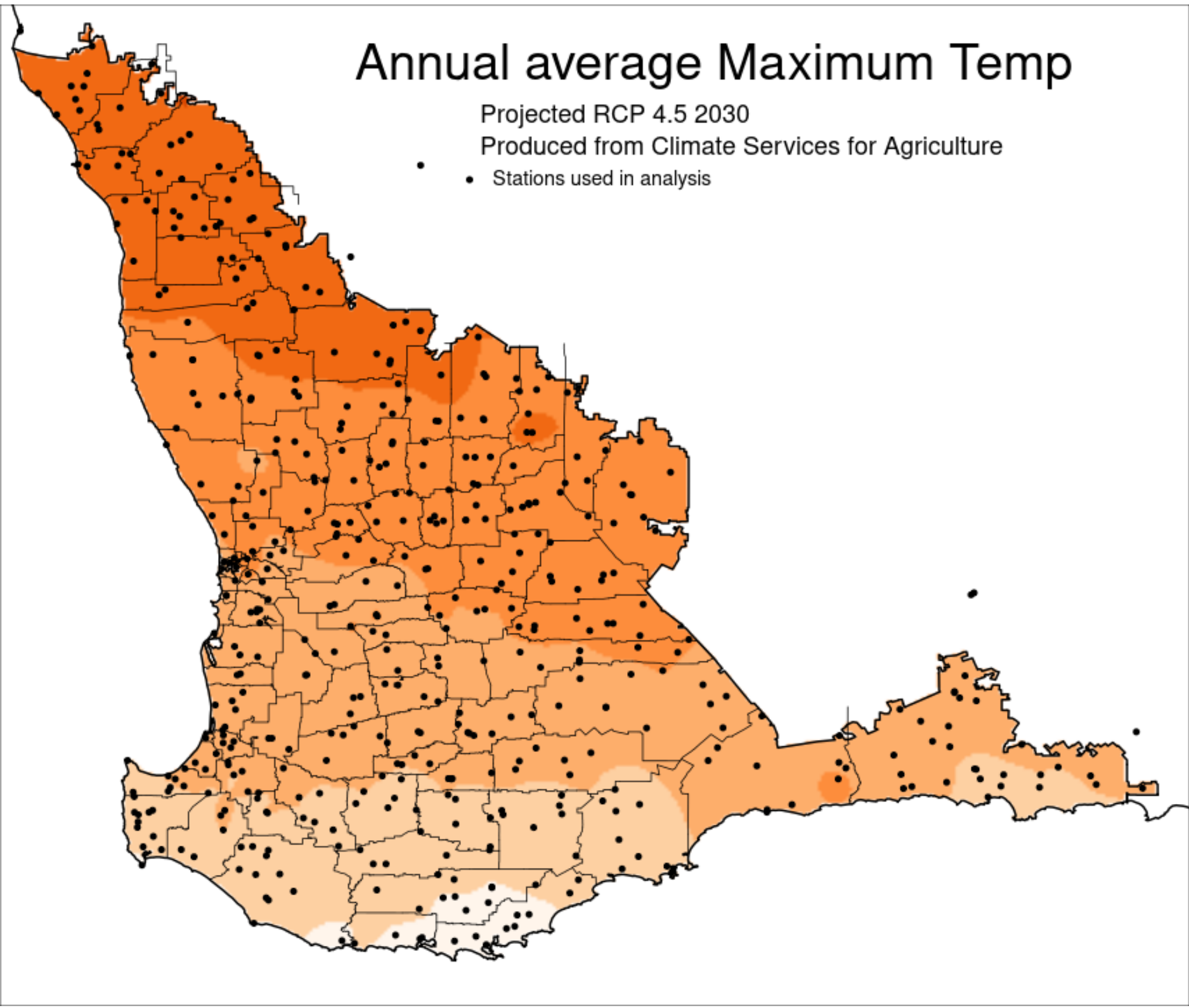
RCP 4.5 2030
